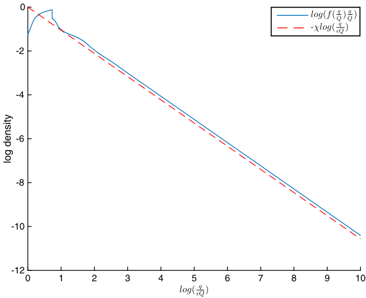
Fig. 1. Stationary distribution.
